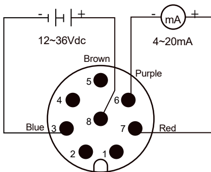
4~20mA output
